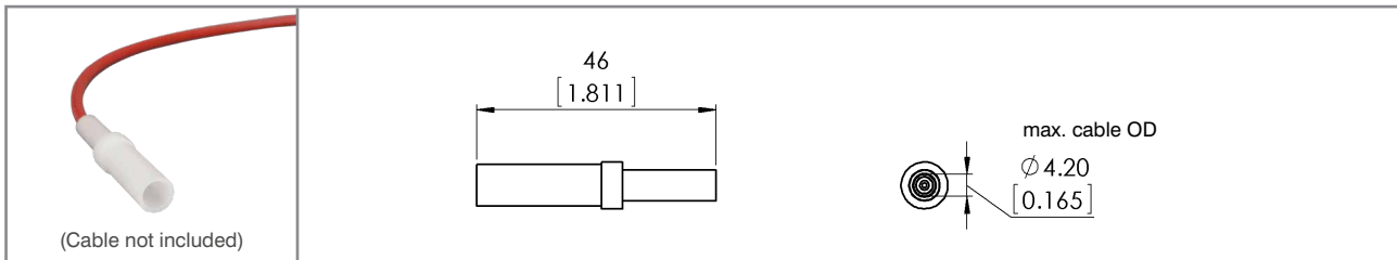
drawing - dimensions in mm [inch]
