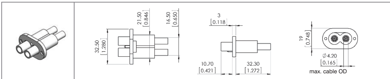
drawing - dimensions in mm [inch]
